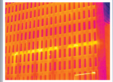
Heat Loss
